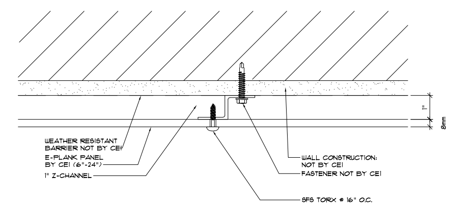
3 VERTICAL MID PANEL DETAIL SCALE: 3" = 1'-0"
