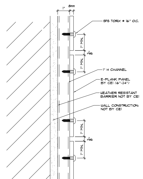
2 HORIZONTAL JOINT DETAIL SCALE: 3" = 1'-0"
