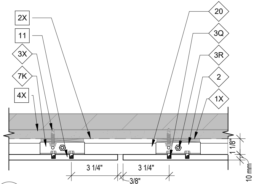
2 C2000 VERTICAL JOINT DETAIL O405 SCALE: 3" = 1'-0"
